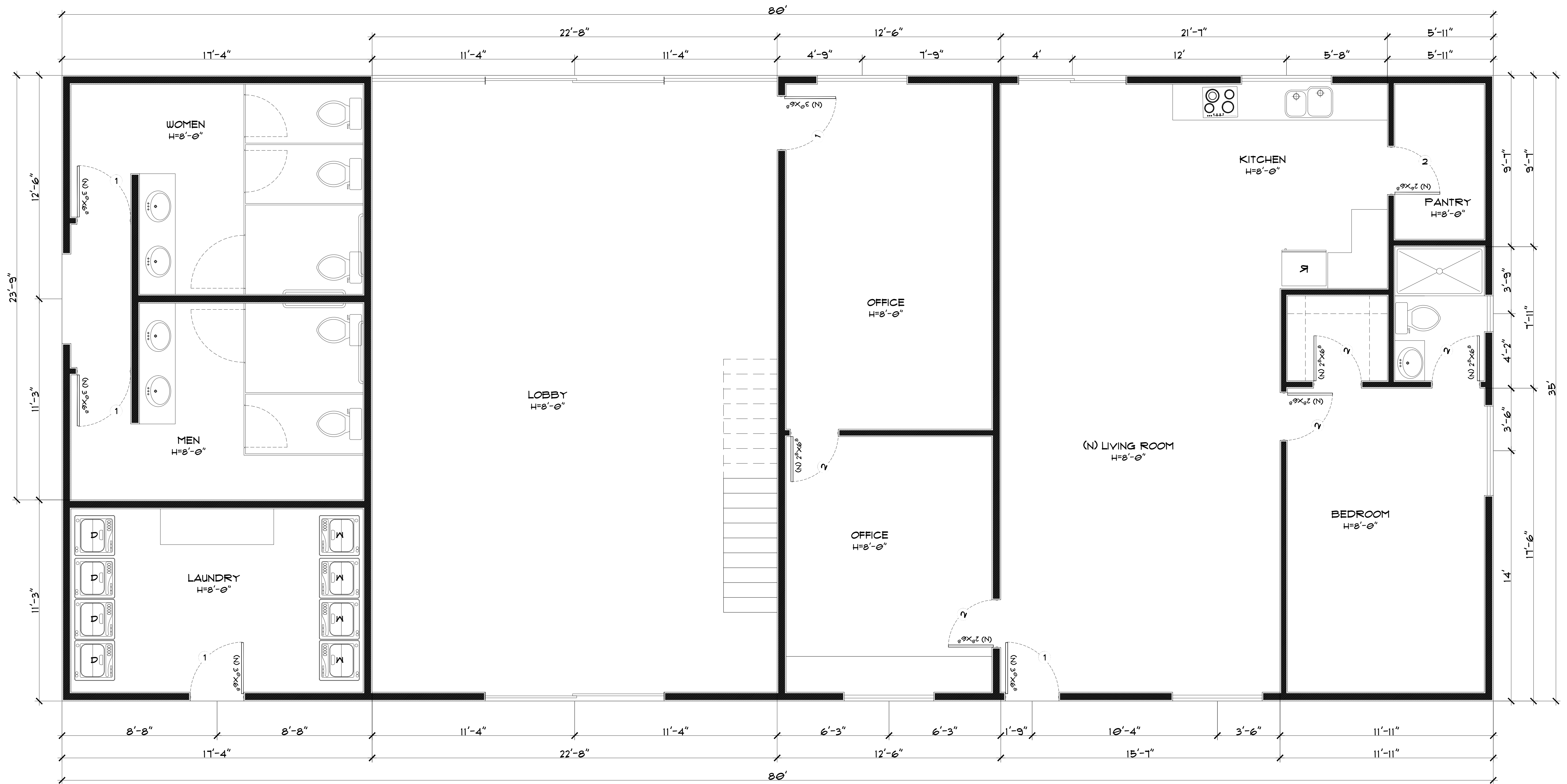
FLOOR PLAN 1ST FLOOR
