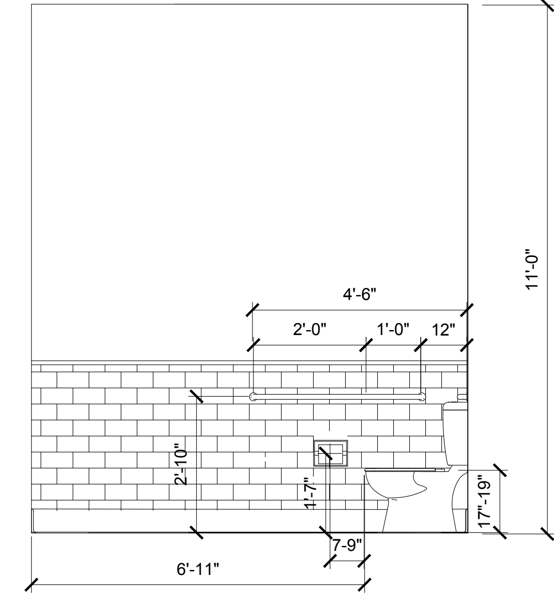
ADA BATHROOM ELEVATIONS 1/2" = 1'-0"
