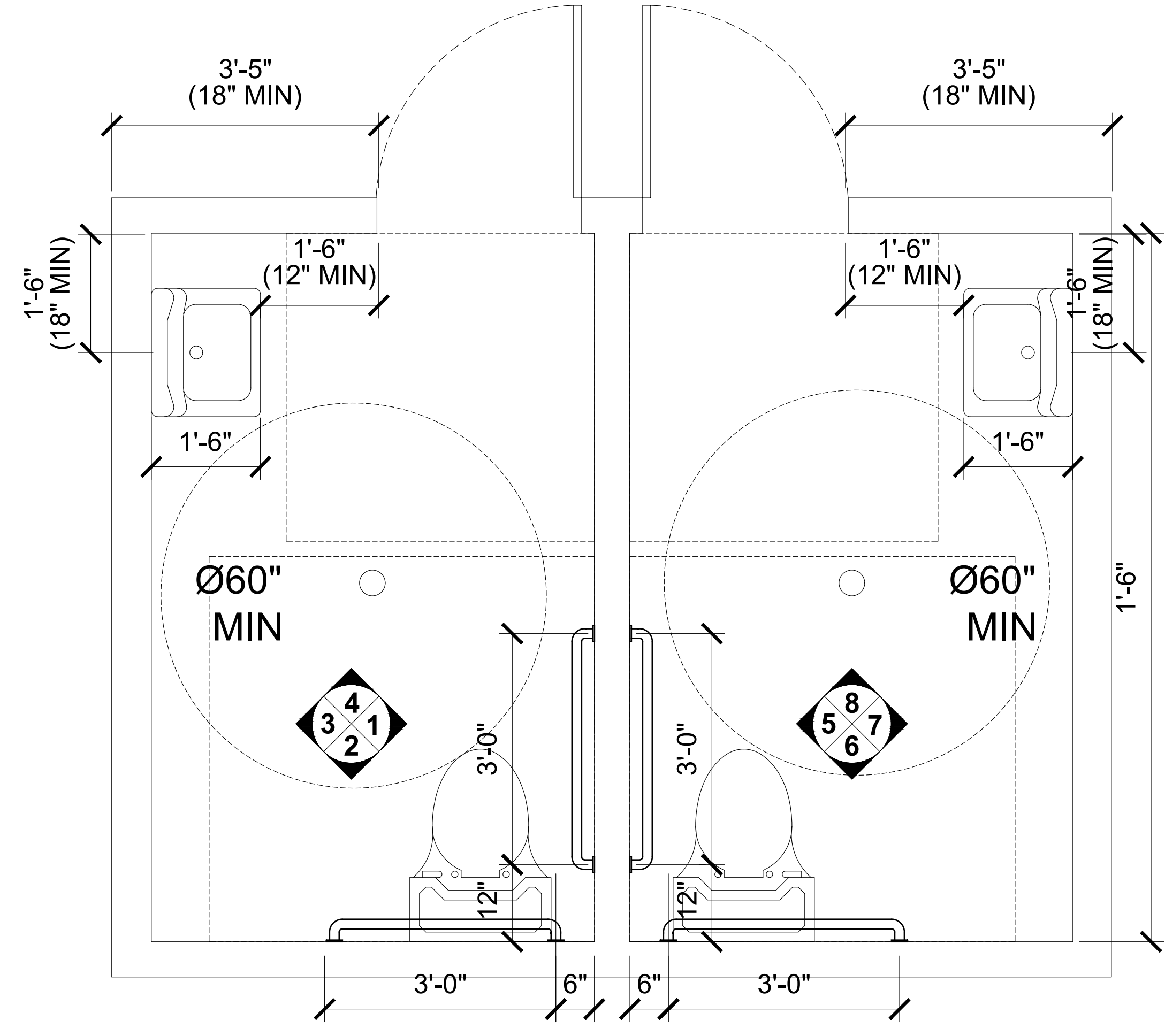
ENLARGED BATHROOM PLAN 3/4" = 1'-0" 9
