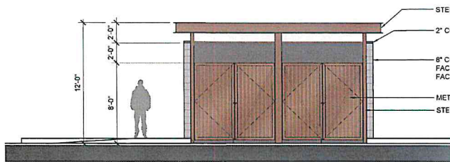
3 FRONT ELEVATION SCALE: 1/4" = 1'-0"
