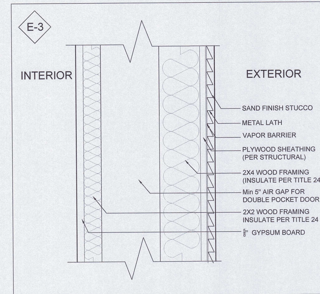
3 EXTERIOR POCKET DOOR WALL SCALE: 3" = 1'-0"
