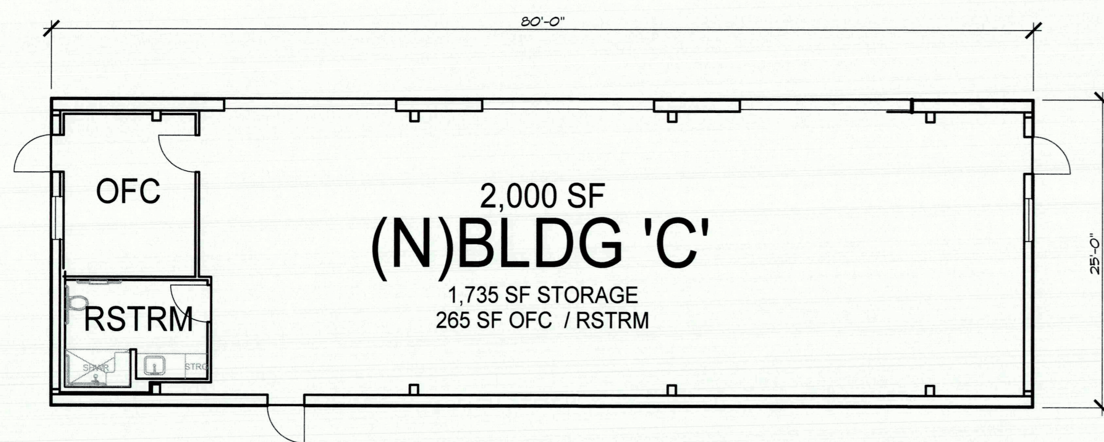
BLDG 'C': FLOOR SCALE: 3/16"=1'-0"
