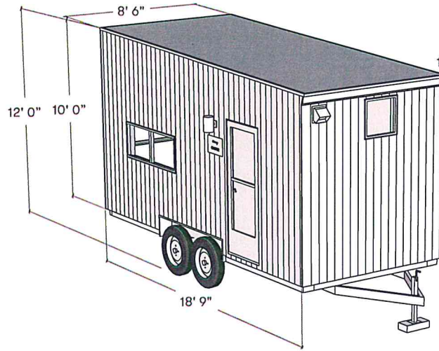
4-Person Cabin
