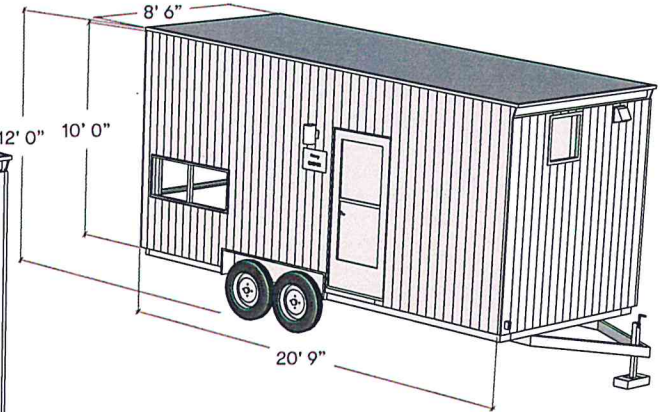
Accessible Cabin
