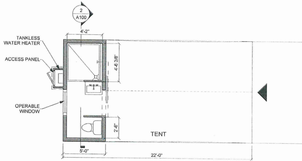
1 BATHROOM/TENT PLAN SCALE: 1/4" = 1'-0"
