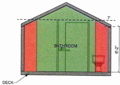
2 SECTION - HGT. DIAGRAM SCALE: 1/4" = 1'-0"
