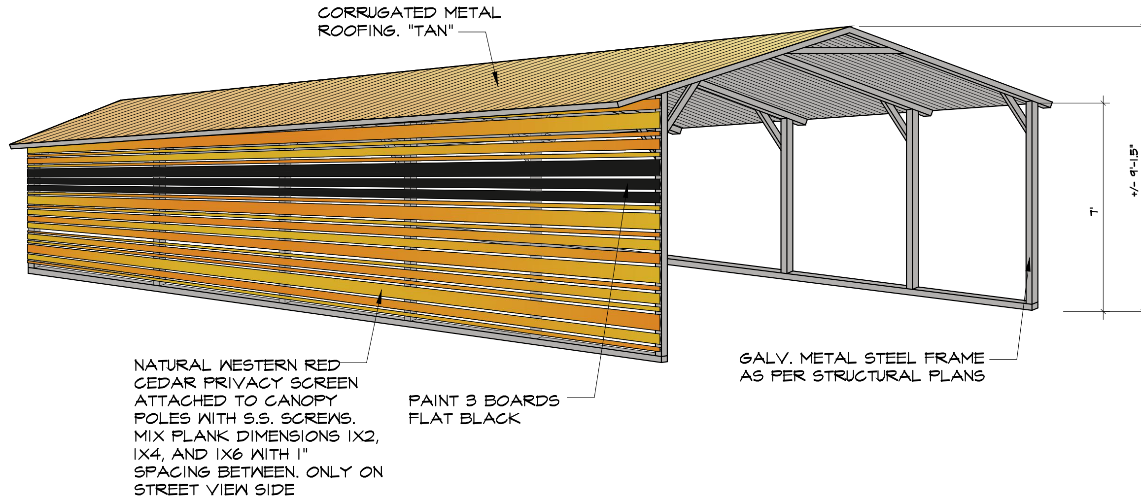
CANOPY ISOMETRIC
