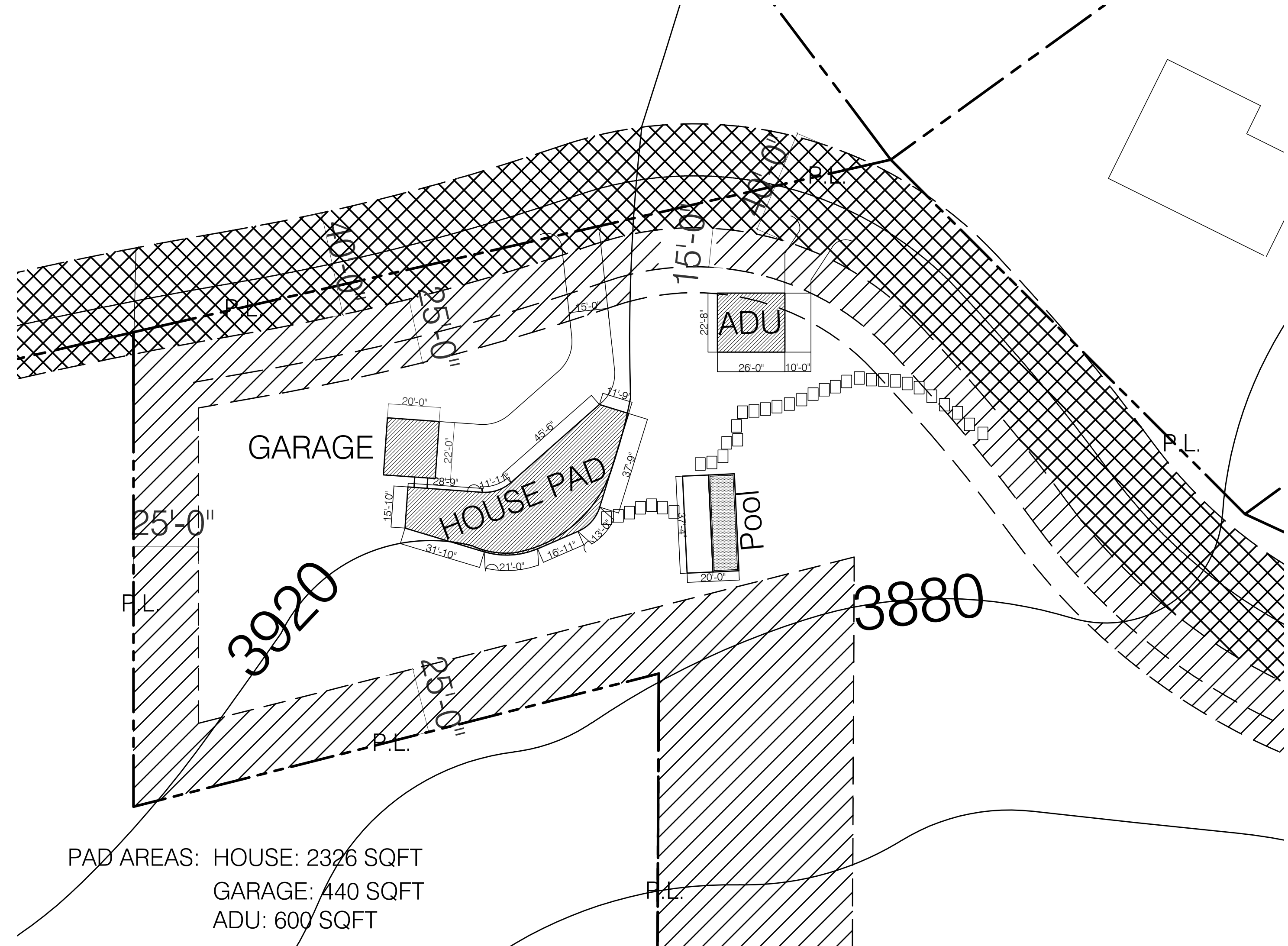
2 PROPOSED SETBACKS SCALE: 1/32" = 1'-0"
