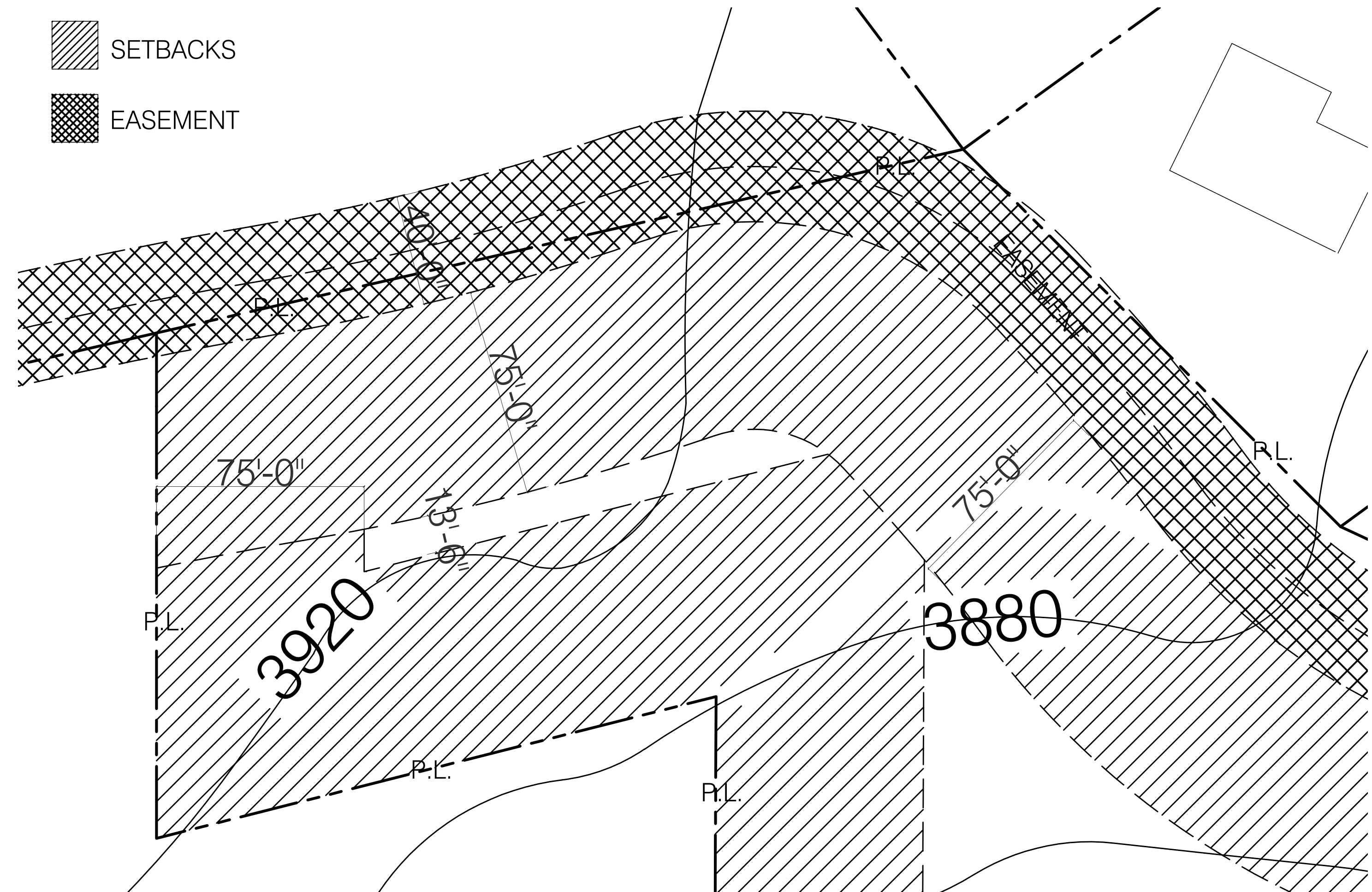
1 EXISTING SETBACKS SCALE: 1/32" = 1'-0"
