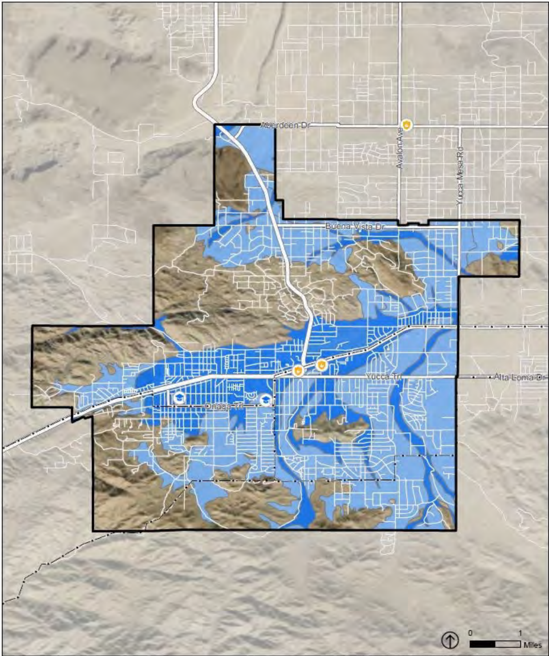
Figure S-3 Seismic Hazard Program Liquefaction Zone
