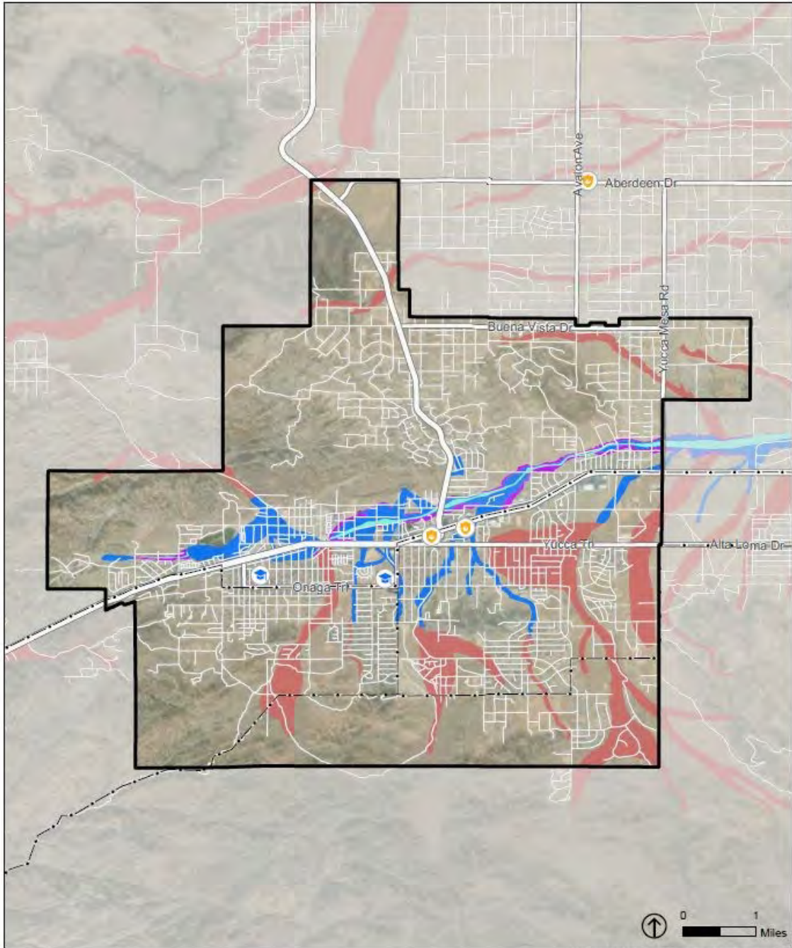
Figure S-4 Flood Hazard Zones
