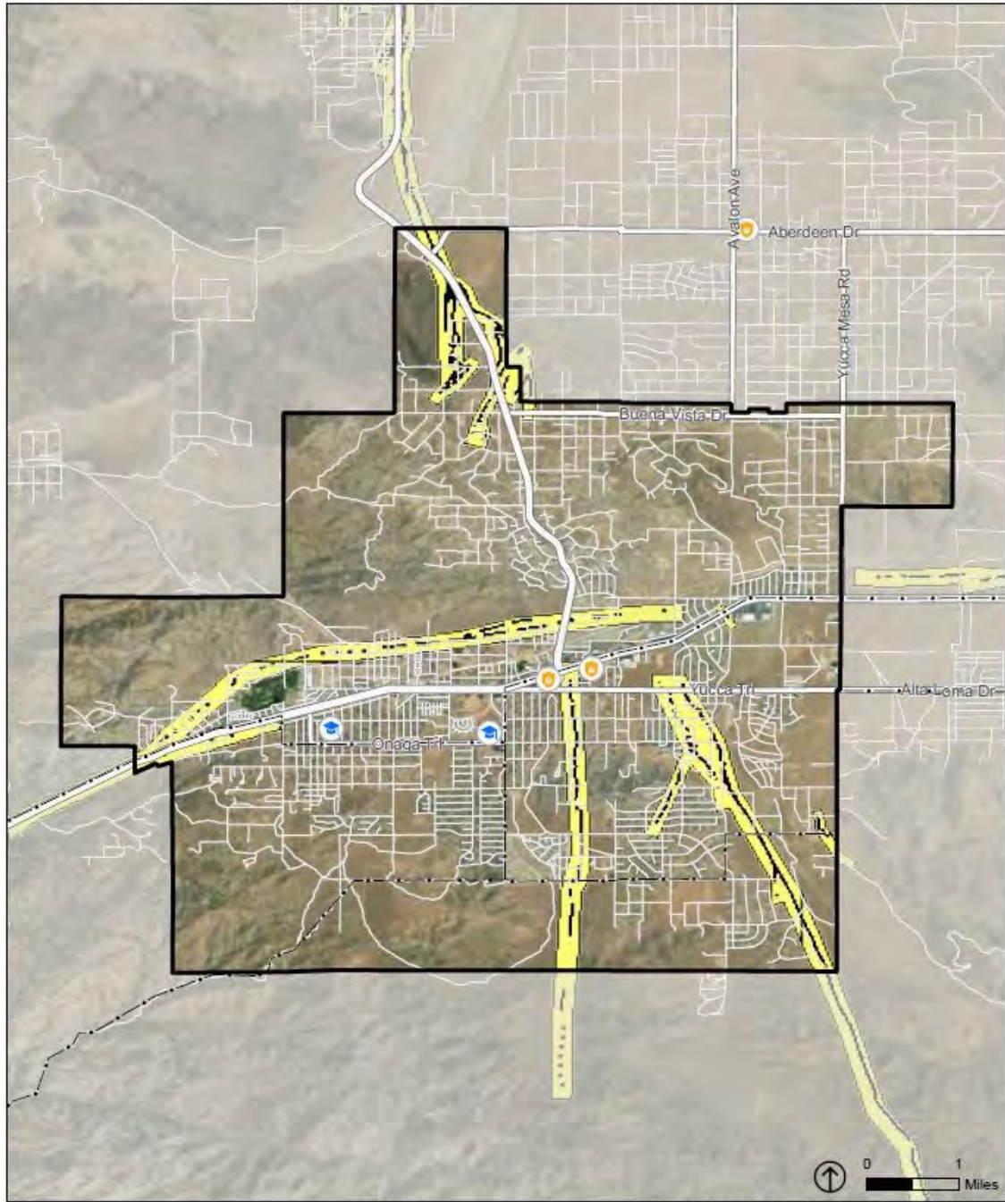
Figure S-2 Regional Fault Zones and Traces
