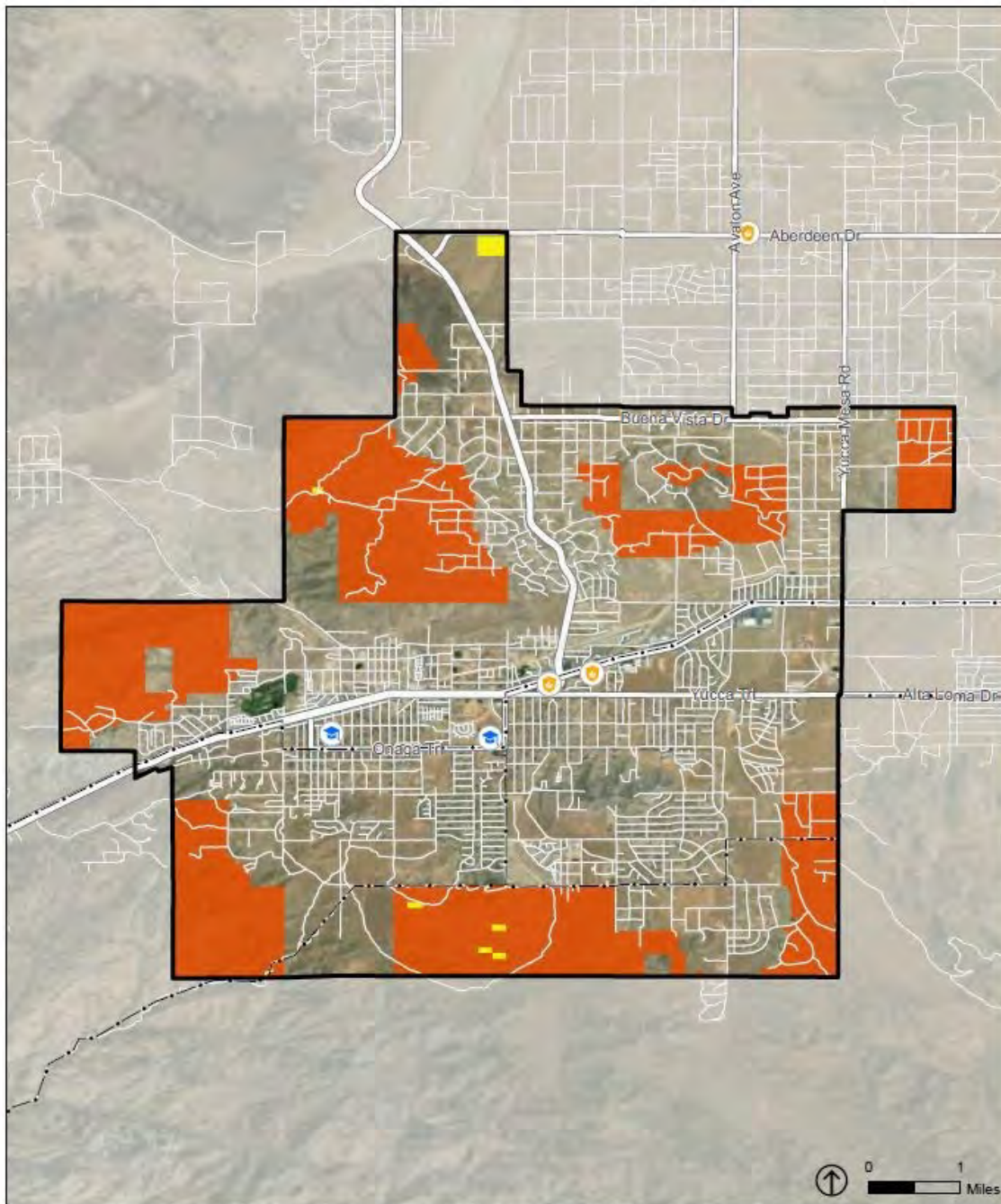
Figure S-8 Residential Parcels with Evacuation Constraints
